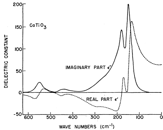
FIG. 6. Real and imaginary part of the dielectric constant of CaTiO 3 obtained from the reflectivity data in Fig. 3.
