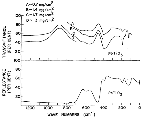
FIG. 2. The infrared transmittance and reflectance spectra of PbTiO 3 from 1250 to 5 cm -1 .
