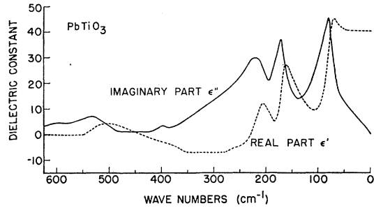
FIG. 5. Real and imaginary part of the dielectric constant of PbTiO 3 obtained from the reflectivity data in Fig. 2.
