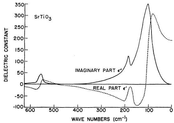
FIG. 4. Real and imaginary part of the dielectric constant of SrTiO 3 obtained from the reflectivity data in Fig. 1.
