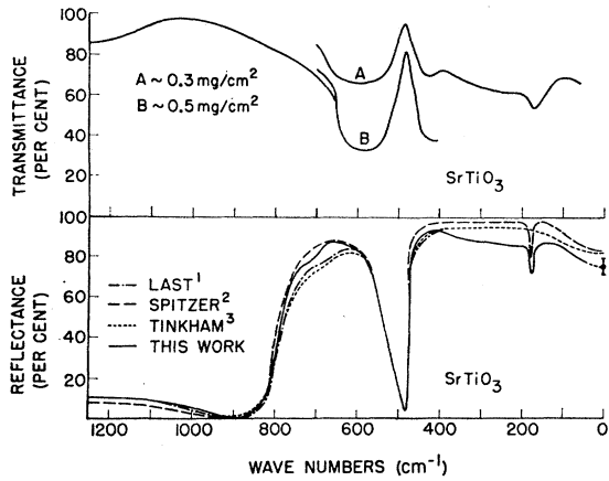
FIG. 1. The infrared transmittance and reflectance spectra of SrTiO 3 from 1250 to 5 cm -1 .
