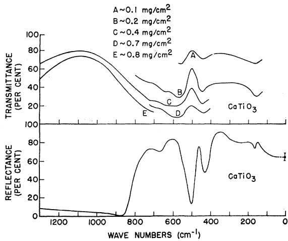
FIG. 3. The infrared transmittance and reflectance spectra of CaTiO 3 from 1250 to 5 cm -1 .
